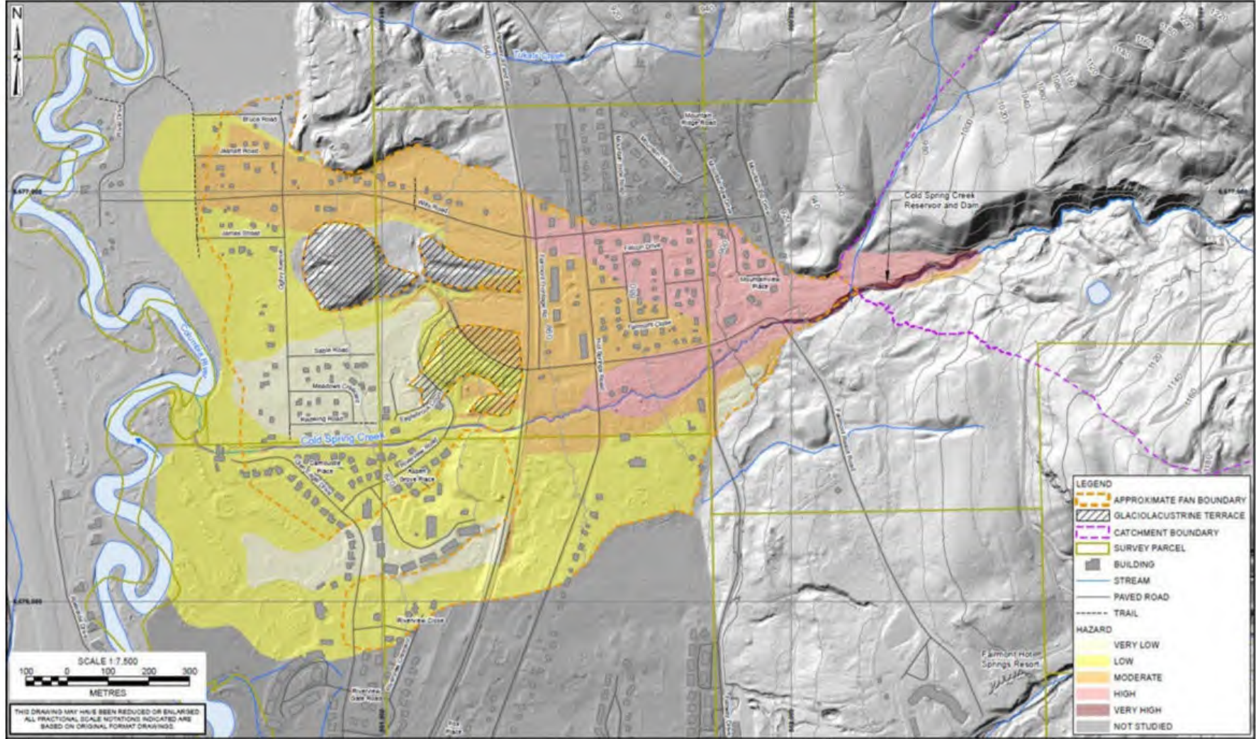
Figure H - 1: Example of a composite hazard map showing different hazard zones defined by impact force x frequency
